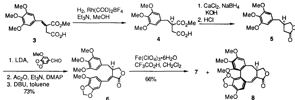
Scheme 2. Synthesis of the optically pure tetracyclic lactone ( 7 )
