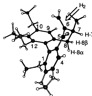
Figure 1. Expected conformation of 12 and stereochemical course of hydrogenation
