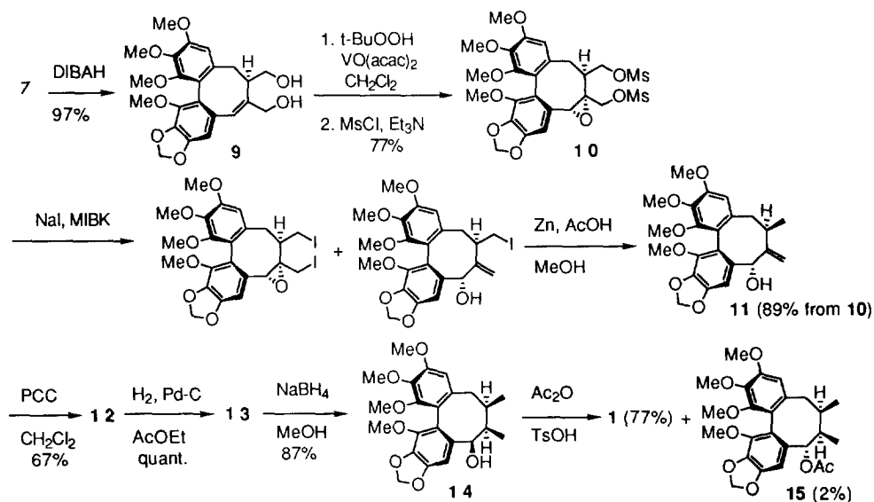
Scheme 3. Total synthesis of kadsurin (1)
