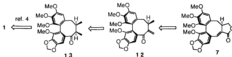
Scheme 1. Synthetic Strategy of 1
